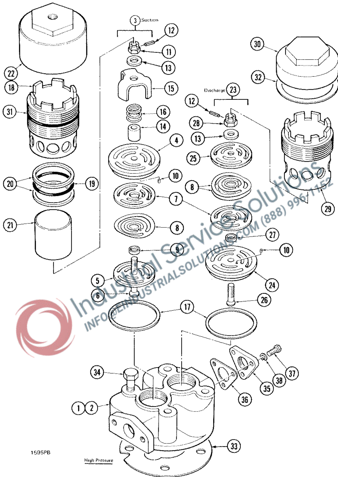
Group 3A Cylinder Head, High Pressure
