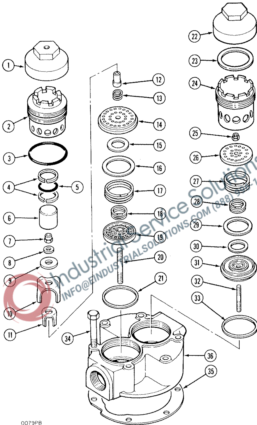
Group No. 2 Cylinder Head, Low Pressure (Right Hand)
