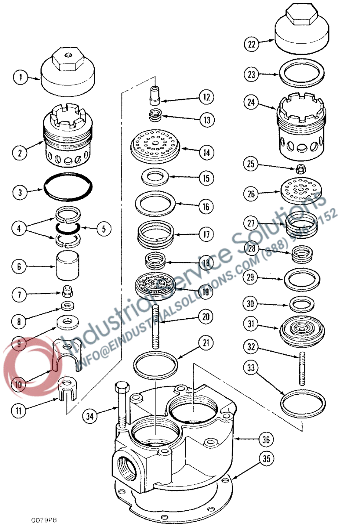
Group No. 2C Cylinder Head, Low Pressure (Left Hand)
